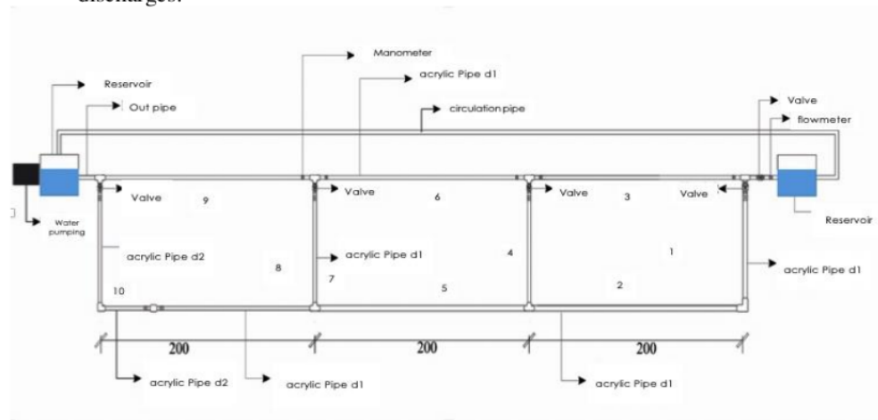
Figure 1. Set Up of Test Equipment.
